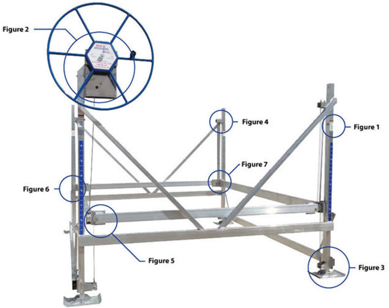
Detail Diagram of the Dock Rite Vertical Boat Lift
